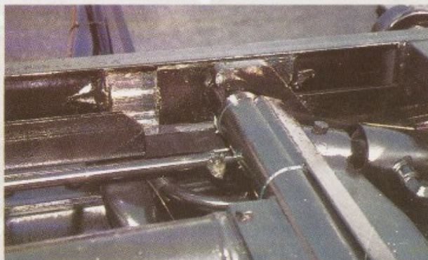
FULL LENGTH SUBFRAME WITH ROLLERS ON BRONZE BUSHINGS AND AUTOMATIC HYDRAULICALLY OPERATED LATCHING DEVICE.
