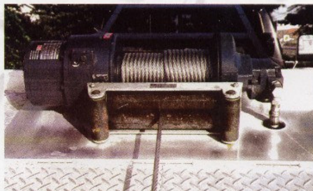
RAMSEY 8000 LB. PLANETARY WINCH & ROLLER CABLE GUIDE.
